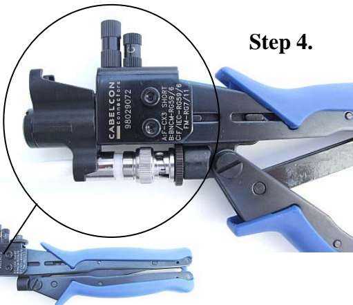
CX3 All Size compression tool item no. 98029072
